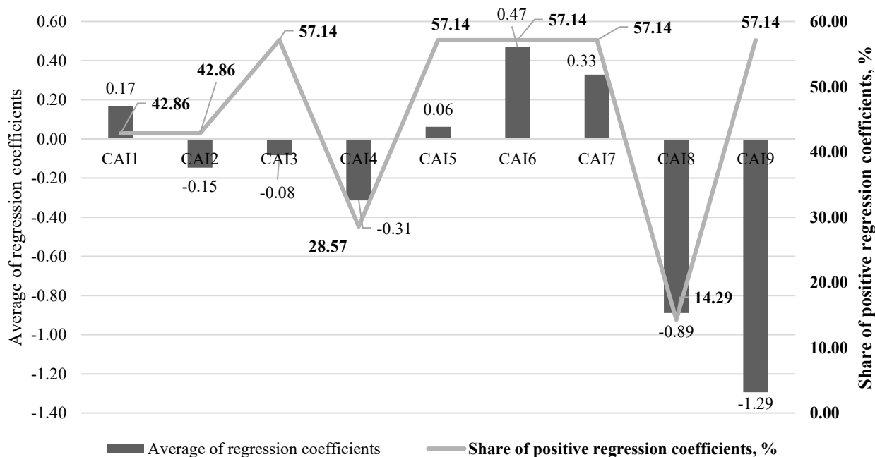
Figure 1. Generalized results of regression analysis.
